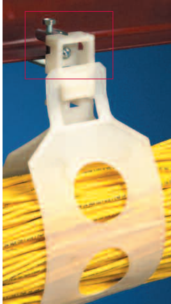
SINGLE LOOP Vertical mounting on beam clamp
