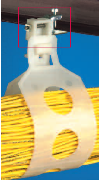
SINGLE LOOP Horizontal mounting on beam clamp
